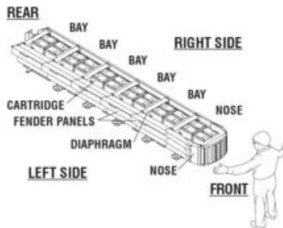
Figure 3 - Orientation
