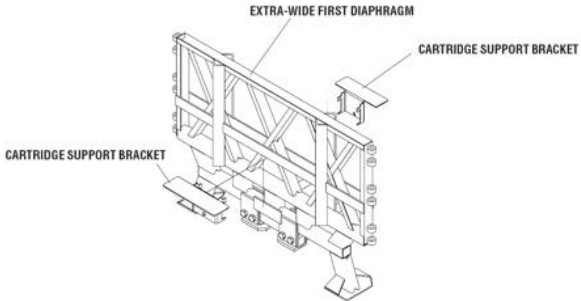
Figure 67 Extra-Wide First Diaphragm
