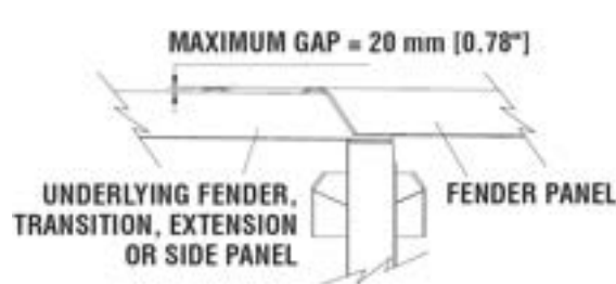
Figure 72 Narrow Systems Fender Panel Gap
