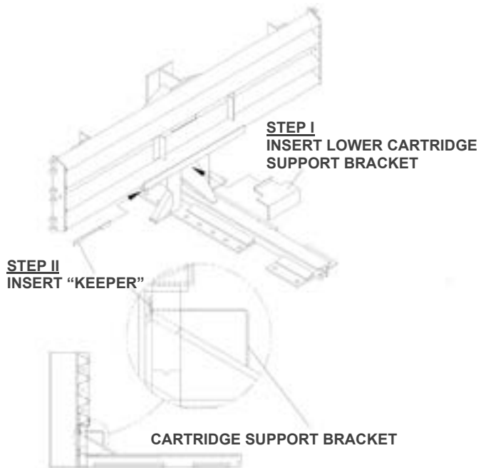
Figure 65 Cartridge Support Bracket (Tension Strut Backup)
