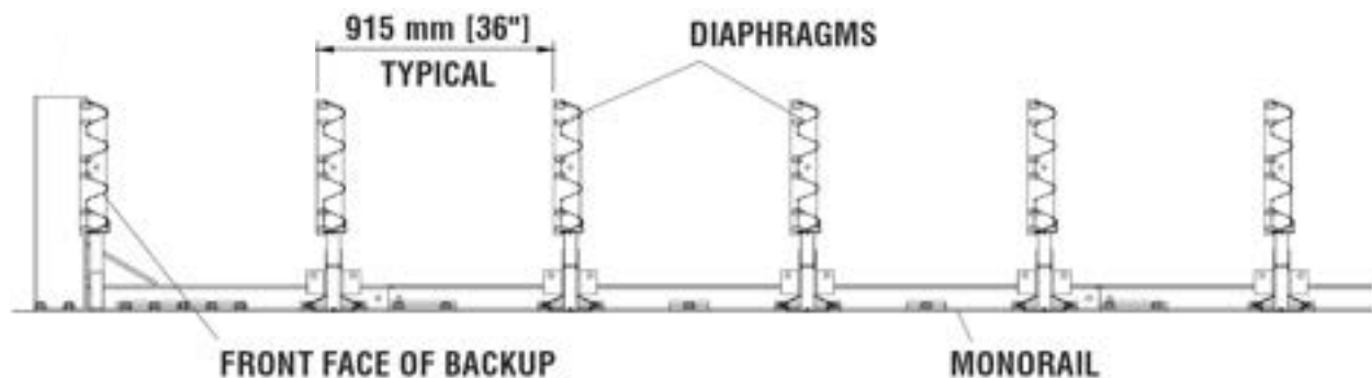
Figure 25 Diaphragm Spacing
